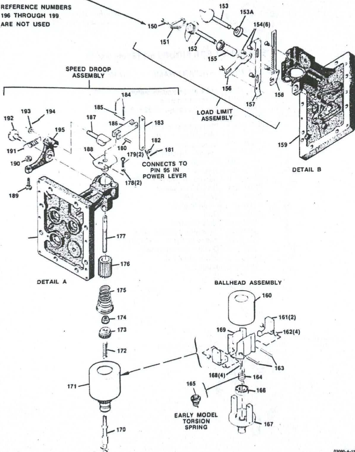
Figure 6-1. Parts Illustration for the UG Dial Governor (Sheet 3 of 5)
