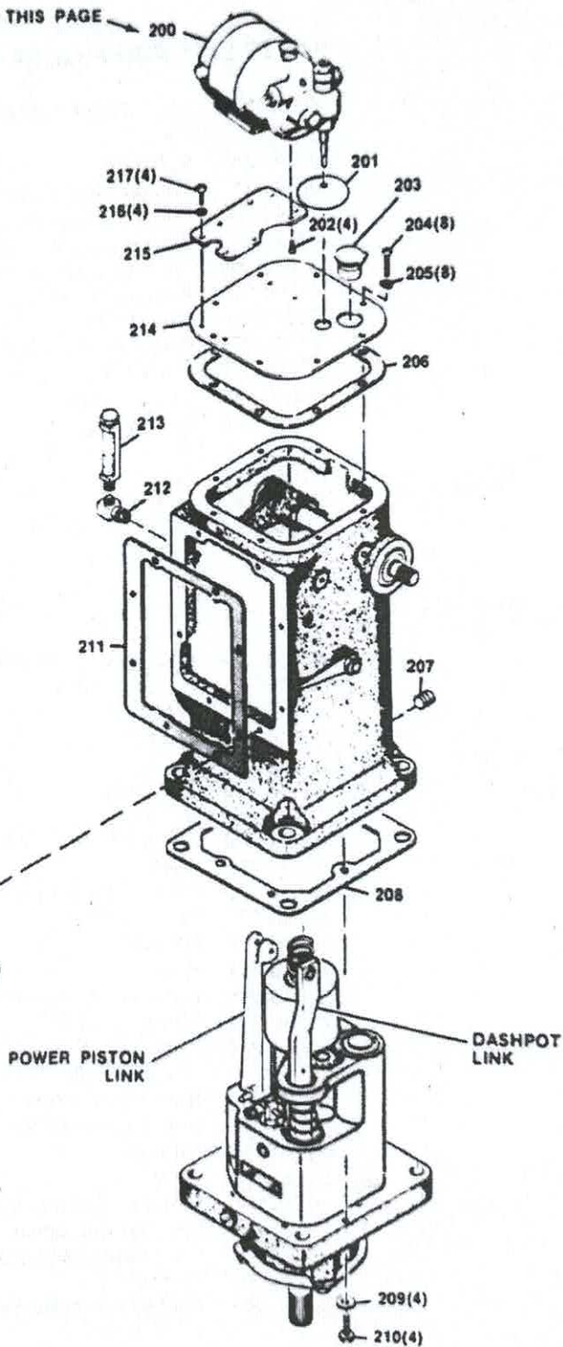
Figure 6-1. Parts Illustration for the UG Dial Governor (Sheet 4 of 5)
