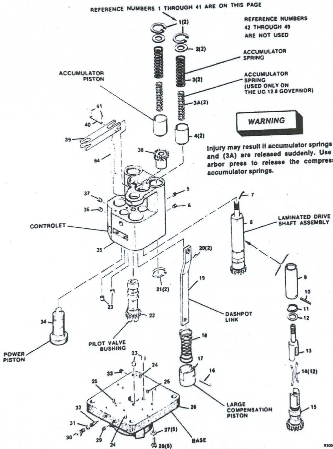
Figure 6-1. Parts Illustration For The UG Dial Governor (Sheet 1 of 5)
