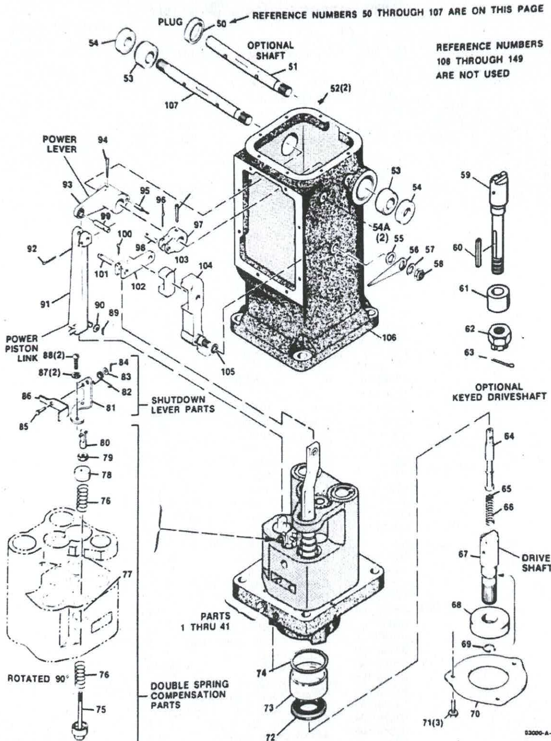
Figure 6-1. Parts Illustration for the UG Dial Governor (Sheet 2 of 5)
